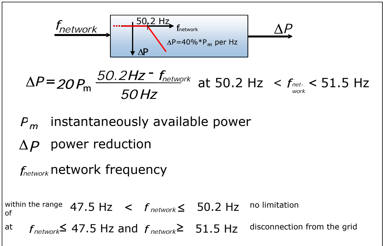
Fig. 3.4: Active power reduction of renewables-based generating units in the case of over-frequency
