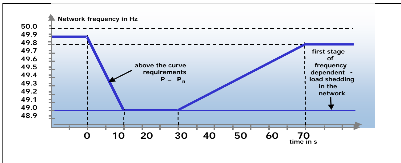
Fig. 3.2: Requirements upon the output from generating units fed into the network within the dynamic short-time range
