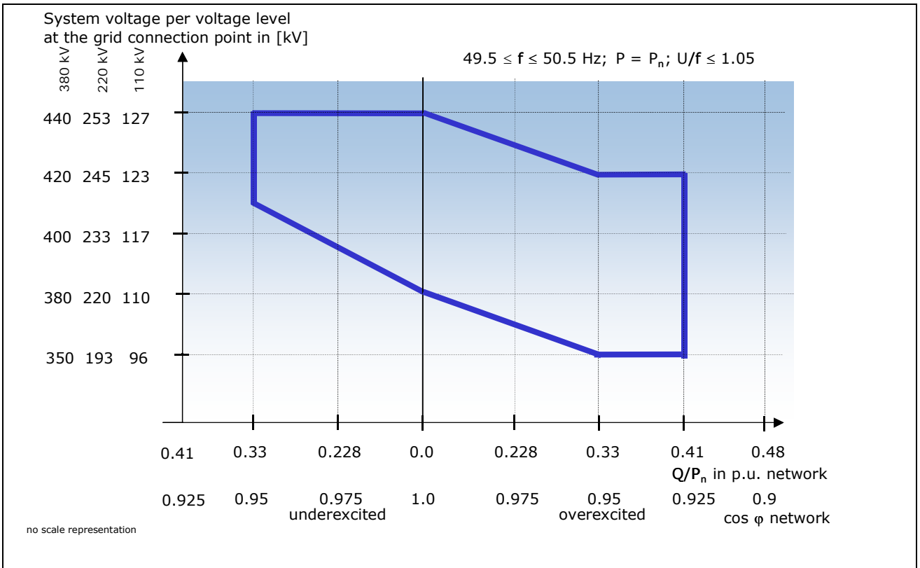
Fig 3.3b: Basic requirement upon the network-side supply of reactive power from generating units to the network (Variant 2)
