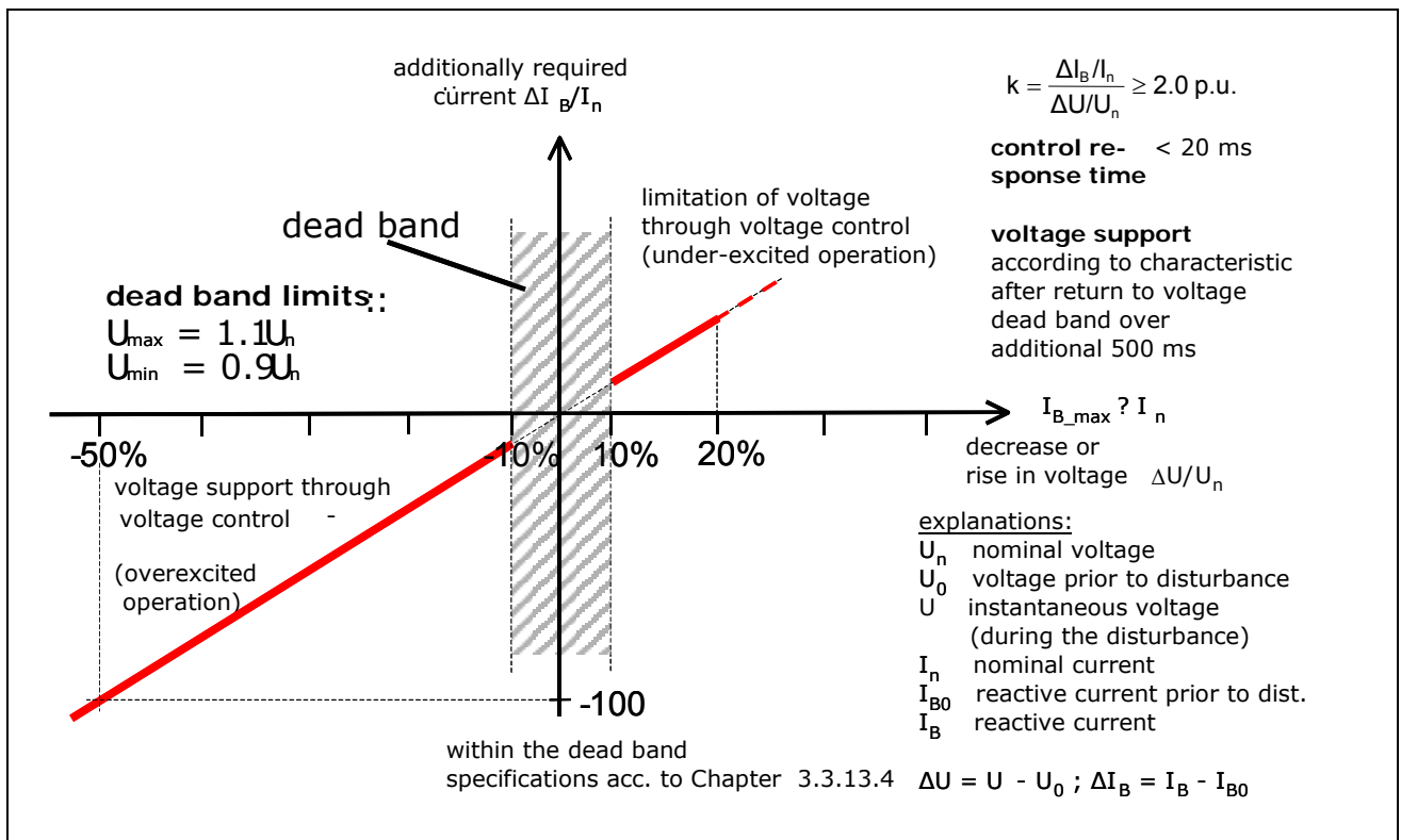
Fig. 3.6: Principle of voltage support in the event of network faults with renewables-based generating facilities
